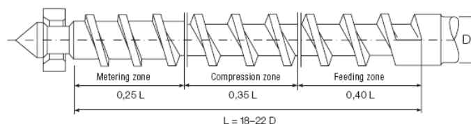
Screw configuration (diagrammatic view)
