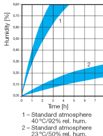
Moisture absorption Polyether-TPU Hardness 80 Shore A – 64 Shore D
